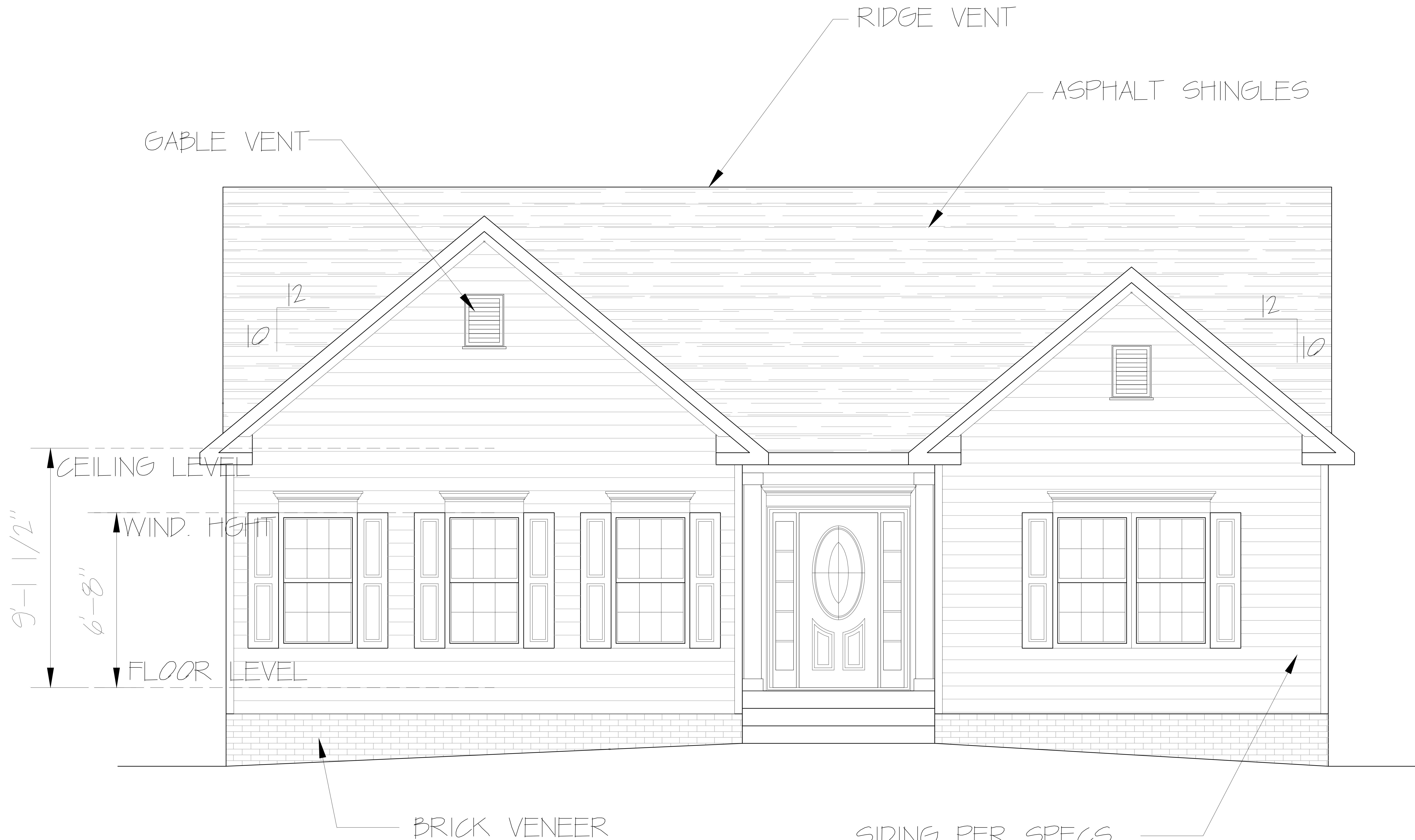
FRONT ELEVATION
