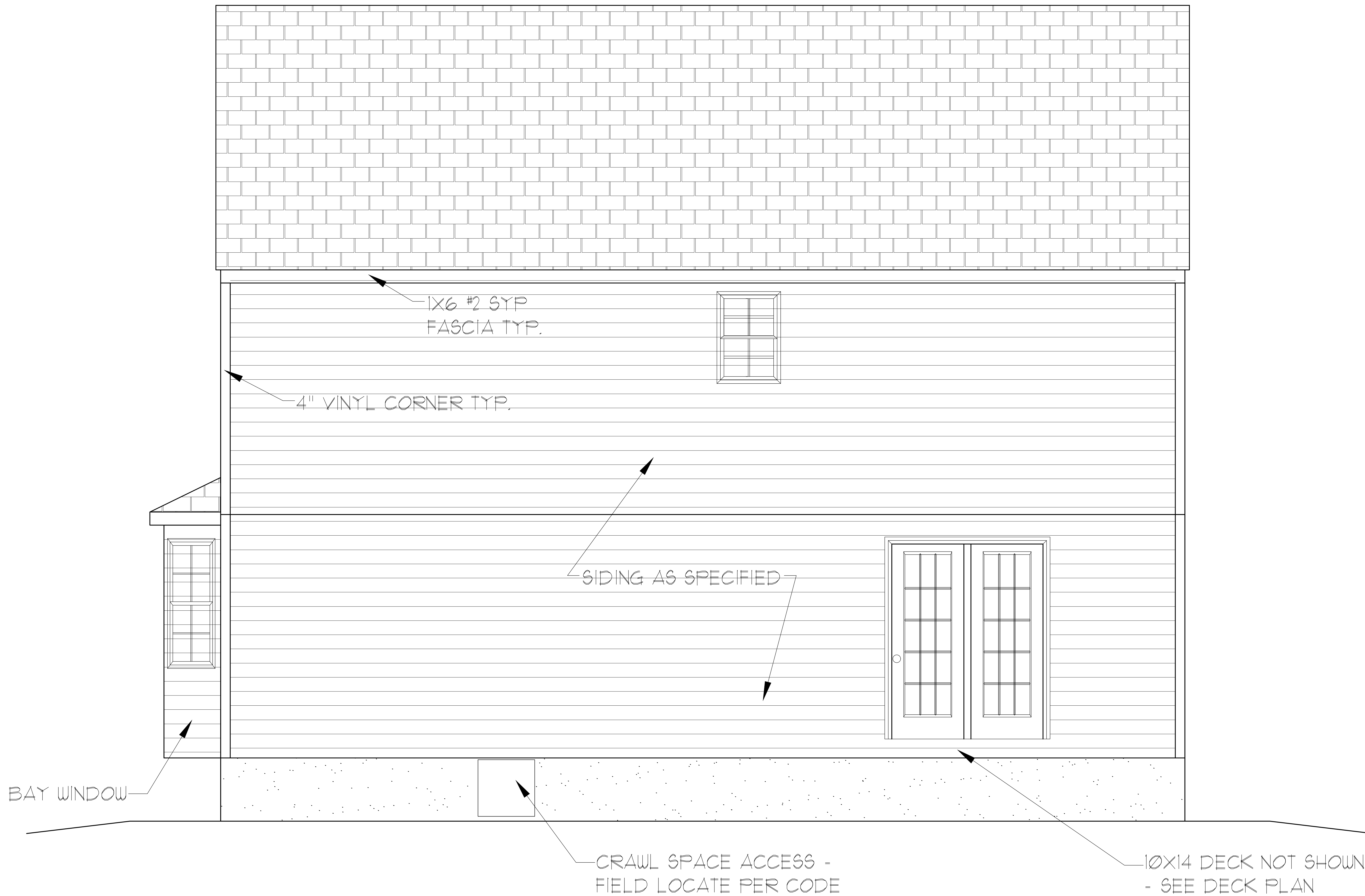
REAR ELEVATION
